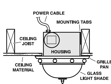
HOUSING MOUNTED DIRECTLY TO JOIST 2x6 (or larger) Discharge parallel to joists.
